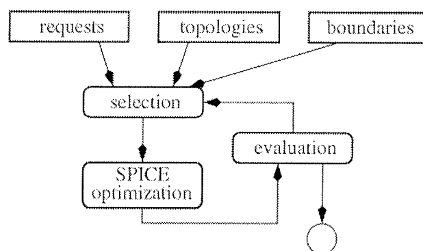
Fig.1: Synthesis of analog circuit
