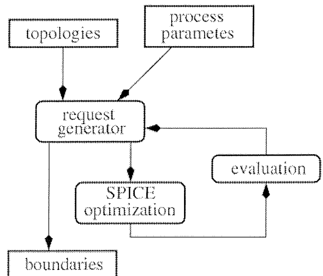
Fig. 2: Topology boundary selection
