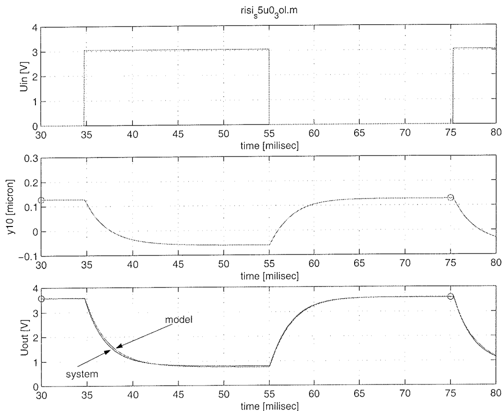
Fig. 4. Open loop system responses in comparison with measurement data (input voltage changes from 0 to 3 V)
