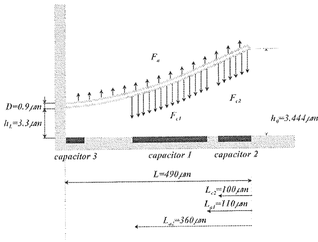
Fig. 1. Schematic system representation
