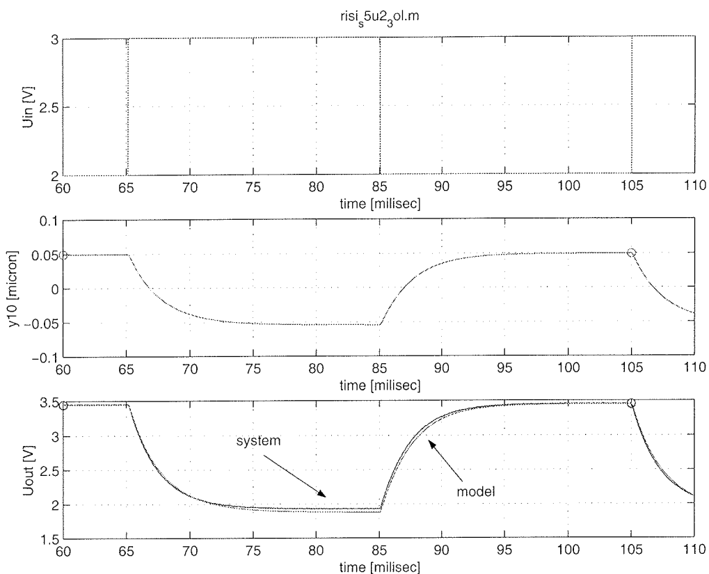
Fig. 5. Open loop system responses in comparison with measurement data (input voltage changes from 2 to 3 V)
