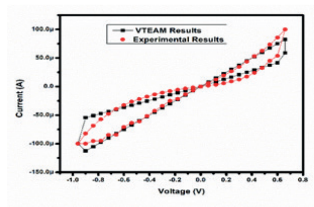
Figure 3: Comparison of Experimental and modelled I-V Characteristics
